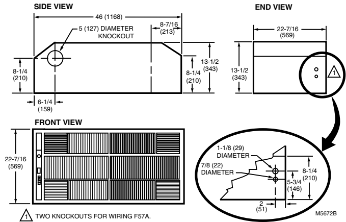
Fig. 1. Approximate dimensions of F57A in. in. (mm).
